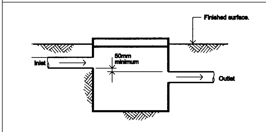
Figure 3.1.2.4 CONSTRUCTION OF SILT PITS
