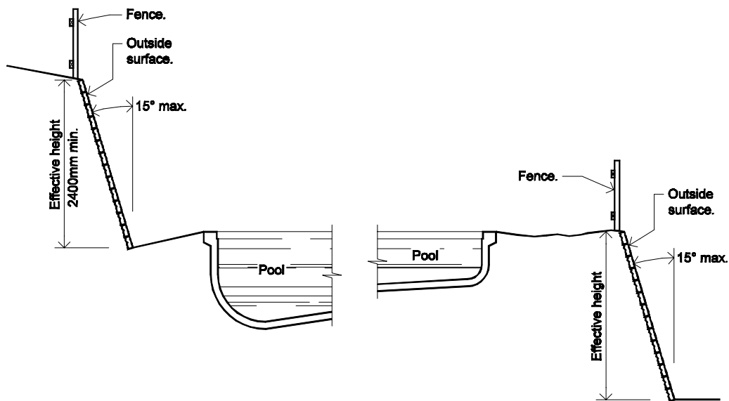
Figure 3.9.3.5 RETAINING WALLS AND OTHER SUCH BARRIERS
