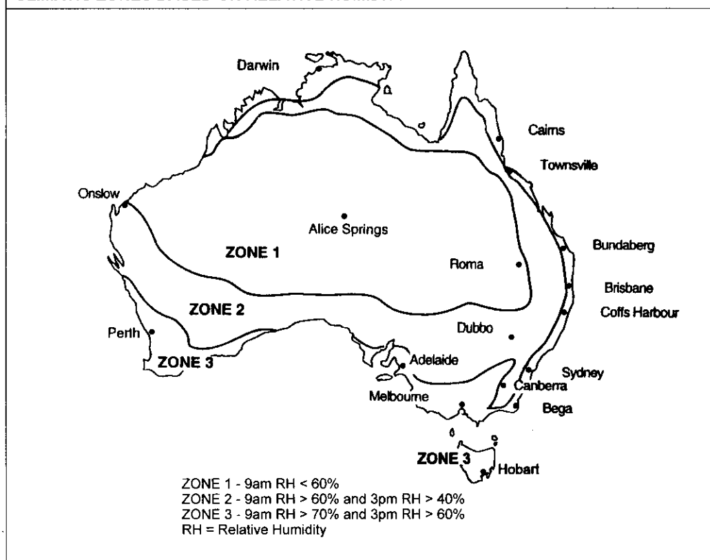
Figure 3.4.1.2 CLIMATIC ZONES BASED ON RELATIVE HUMIDITY
