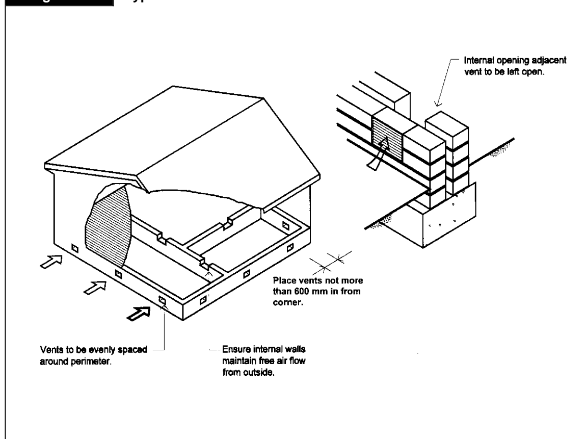
Diagram a. Typical Cross Ventilation Of Sub-Floor Area
